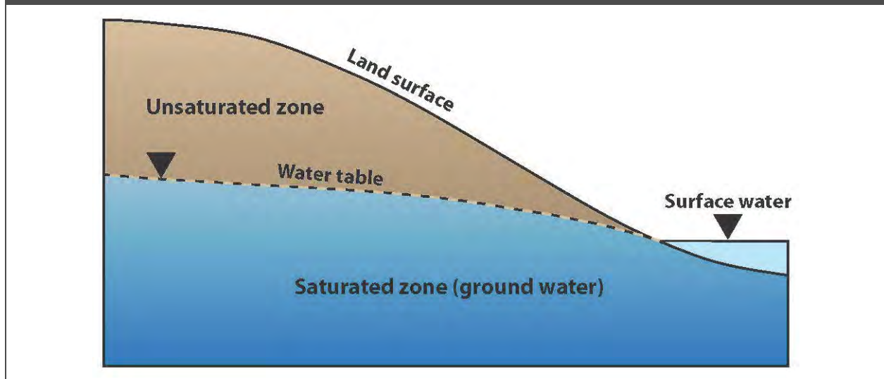
Figure 2-4. Water below the land surface occurs in either the unsaturated or the saturated zone. The upper surface of the saturated zone is the water table. Ground water and ground-water flow occur in the saturated zone. If a surface-water body is connected to the ground-water system, the water table intersects the water body at or near the surface of its shoreline. Modified from Winter et al. (1998).
