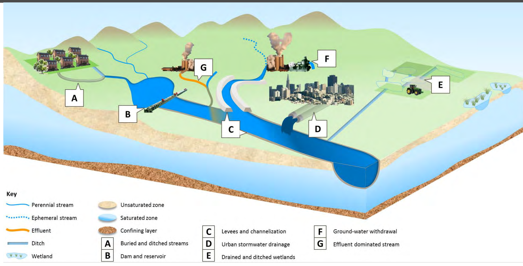
Figure 1-3. Effects of human alterations on watershed connectivity. See Section 1.2.4 for description of alterations illustrated in A-G.
