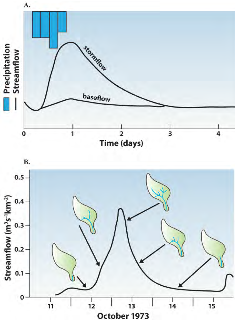
Figure 2-8. (A) Hypothetical hydrograph showing stormflow and baseflow responses to a rainfall event. (B) Expansion and contraction of flowing water in a stream network following a rainfall event. Panel B Source: Reprinted from Subsurface stormflows in the highly permeable forested watersheds of southwestern British Columbia, (1988) by Cheng et al. with permission of Elsevier.
