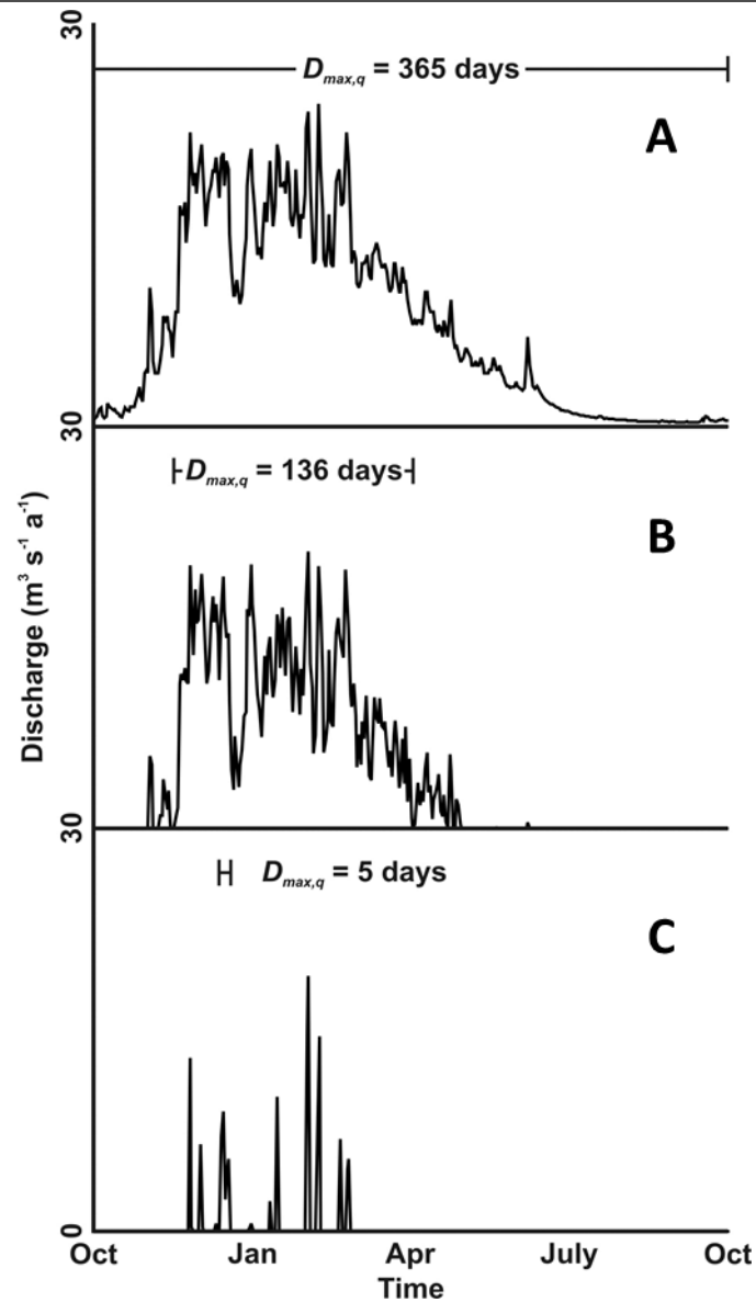
Figure 2-7. Hypothetical hydrographs illustrating maximum duration of flow ( D_{max,q} ) for (A) perennial, (B) intermittent, and (C) ephemeral streams. Source: Reprinted from Non-navigable streams and adjacent wetlands: Addressing science needs following the Supreme Court's Rapanos decision, (2008) by Leibowitz et al. with permission of Ecological Society of America.
