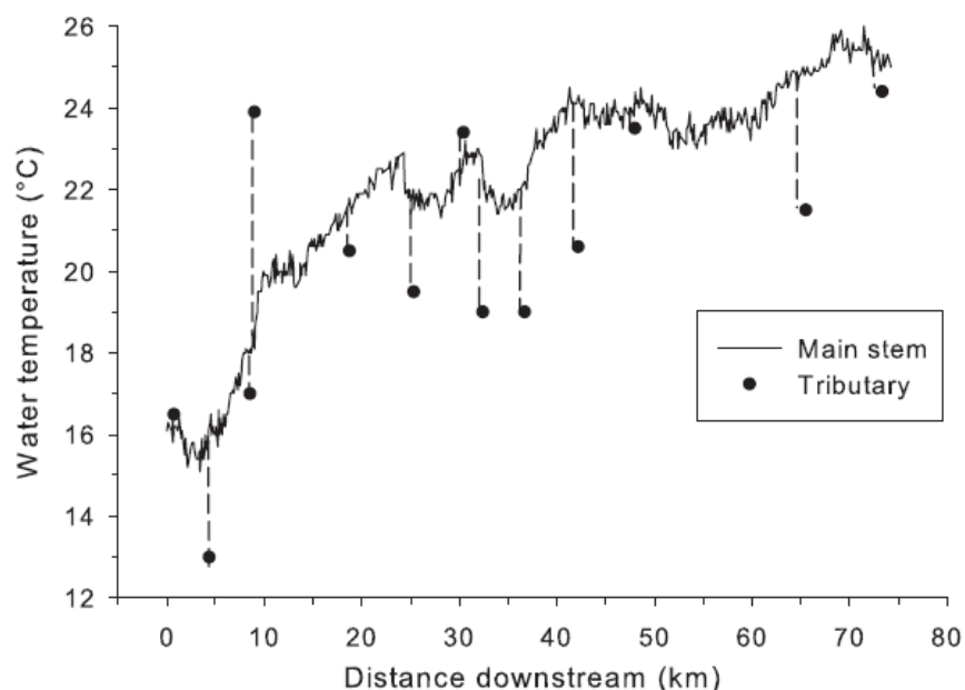
Figure 3-3. Airborne thermal infrared remotely sensed water temperature in the mainstem and at tributary confluences of the North Fork John Day River, OR, on 4 August 1998. Line indicates mainstem, black dots indicate tributary confluences, and dashed vertical lines indicate location of tributary confluences along the mainstem. Reprinted with permission from Torgersen et al. (2008).
