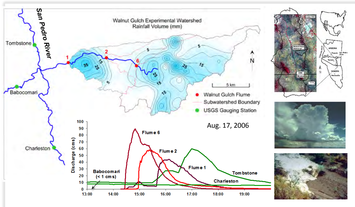
Figure B-10. Storm rainfall and downstream hydrographs with decreasing runoff volume and peak rate due to channel transmission losses as measured by in the USDA-ARS Walnut Gulch Experimental Watershed (WGEW) and the impact of this storm runoff on the San Pedro River in SE Arizona. Inset photos show a typical air-mass thunderstorm and the front of surface flow progressing down an ephemeral channel. Photo of ephemeral stream from Levick et al. (2008).
